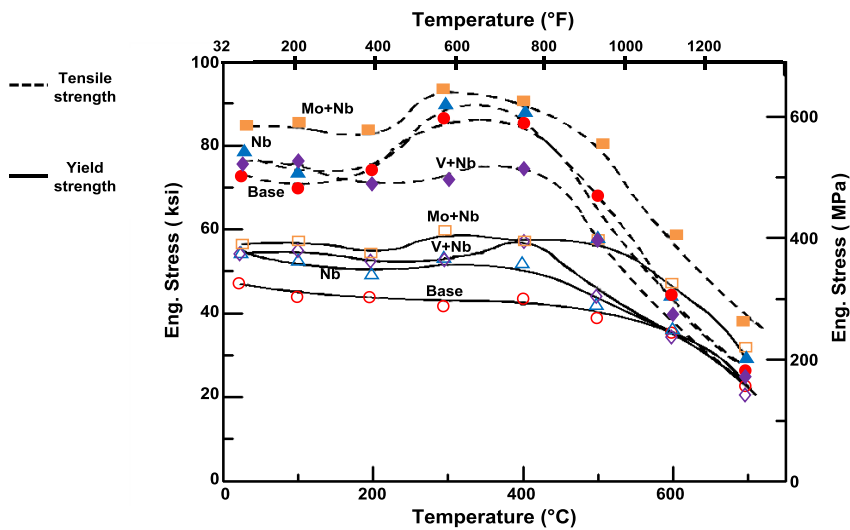
Figure 2. Yield stress (open symbols) and tensile stress (closed symbols) at 25 – 700 °C for base, Nb, Mo+Nb, and V+Nb alloys, tested at an engineering strain rate of 3.9 \times 10^{-3} \text{ s}^{-1} [23].
