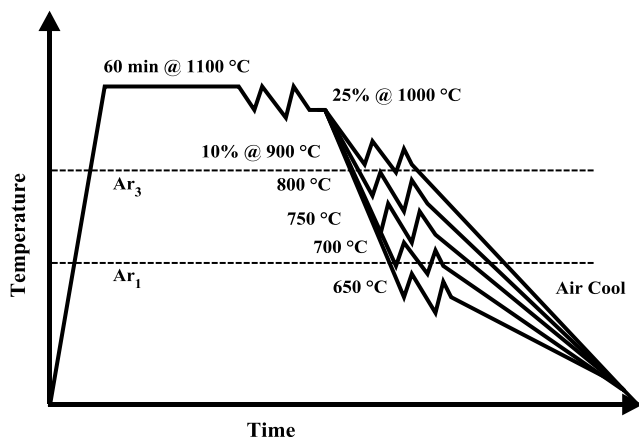
Figure 8. Schematic illustration of thermomechanical processing variations used to examine the influence of warm working in the Nb-containing steel [29].
