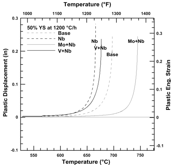
Figure 5. Constant load test results for the base, Nb, Mo+Nb, and V+Nb alloys at 50% yield strength for each alloy and a heating rate of 1200 °C/h. The reduced section of the test specimen was nominally 25.4 mm in length [23].
