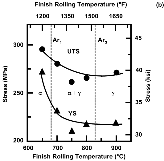
Figure 10. Yield and tensile strengths at room temperature (a) and 600°C (b) for Nb-steel finish rolled (10%) at different temperatures, tested at an engineering strain rate of 3.9 \times 10^{-3} \text{ s}^{-1} [29].
