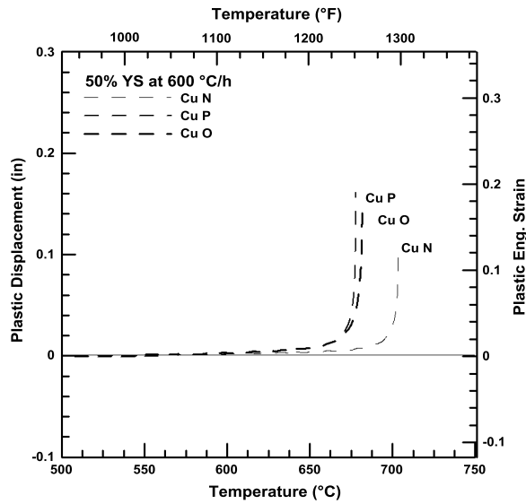
Figure 7. Constant load tests for three Cu alloy conditions: normalized (N), peak-aged (P) and overaged (O) tested at an applied stress equal to 50% of the room temperature yield strength for each condition. The heating rate was 600 °C/h and the reduced section of the test specimen was nominally 25.4 mm in length [23].
