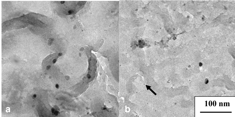
Figure 6. TEM bright field images from carbon extraction replicas showing fine precipitates in the Nb (a) and Mo+Nb (b) alloys after constant load testing at 300 °C/h [3].
