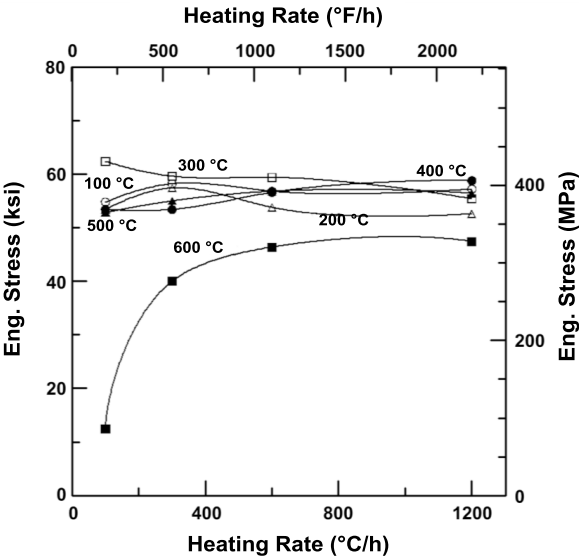
Figure 4. Influence of heating rate (100 – 1200 °C/h) to test temperature on the yield strength of the Mo+Nb alloy. Testing was conducted at an engineering strain rate of about 3.9 \times 10^{-3} \text{ s}^{-1} following a 15 minute holding time at the test temperature [23].
