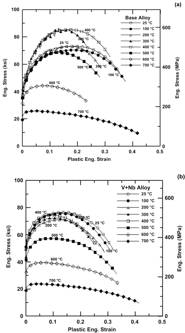
Figure 3. Engineering stress/plastic strain curves for the base (a) and V+Nb (b) alloys at temperatures between 25 and 700 °C, tested at an engineering strain rate of 3.9 \times 10^{-3} \text{ s}^{-1} [23].
