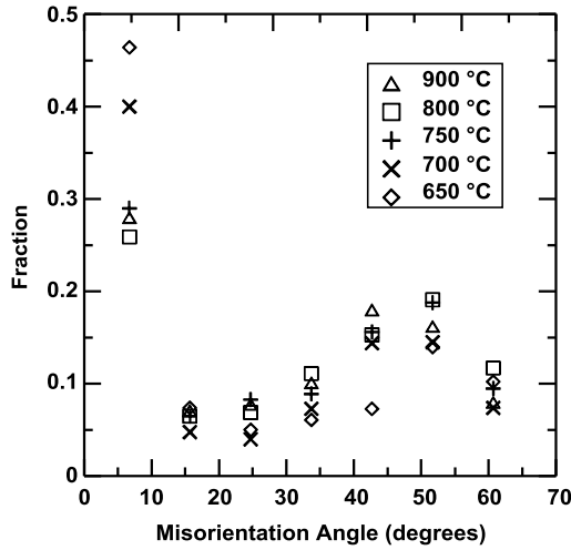
Figure 9. Distribution of misorientation angles for the Nb steel, laboratory rolled using finishing temperatures between 900 °C and 650 °C [30].
