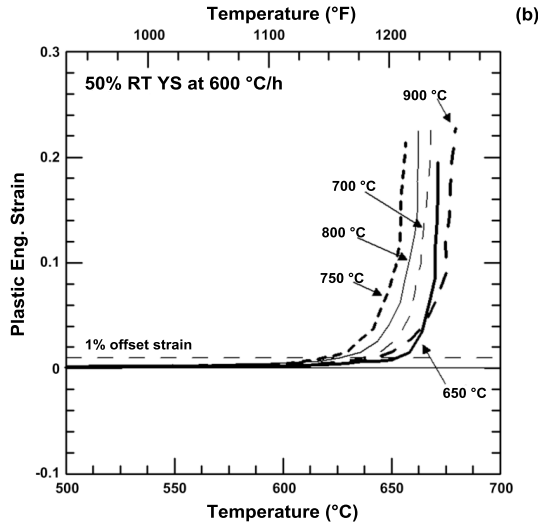
Figure 11. Constant load tests for the Nb-alloy finish rolled 10% at different temperatures (indicated on the figures). The results in (a) are for a constant applied stress (187 MPa), while those in (b) were conducted at an applied stress 50% of the room temperature yield stress for each condition.
