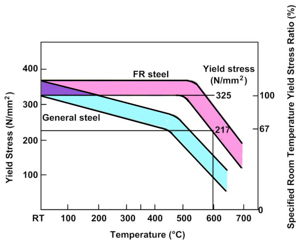
Figure 1. Schematic comparison showing improved elevated temperature strength of FR steel. (Adapted from [2], with permission).
