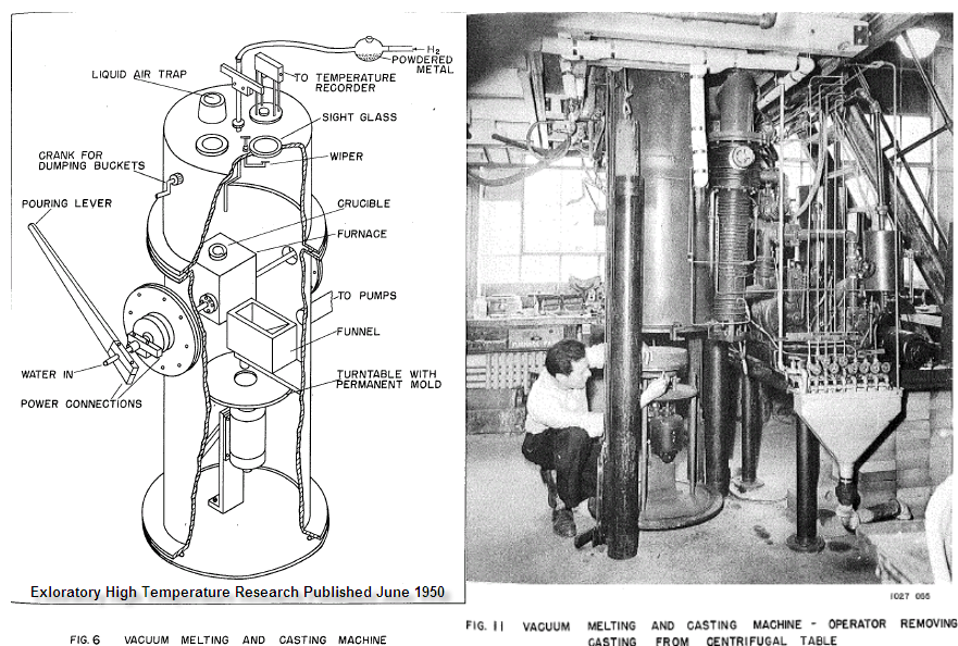
Figure 3. 1950 VIM Schematic and Furnace
